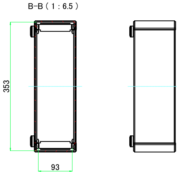
D view
